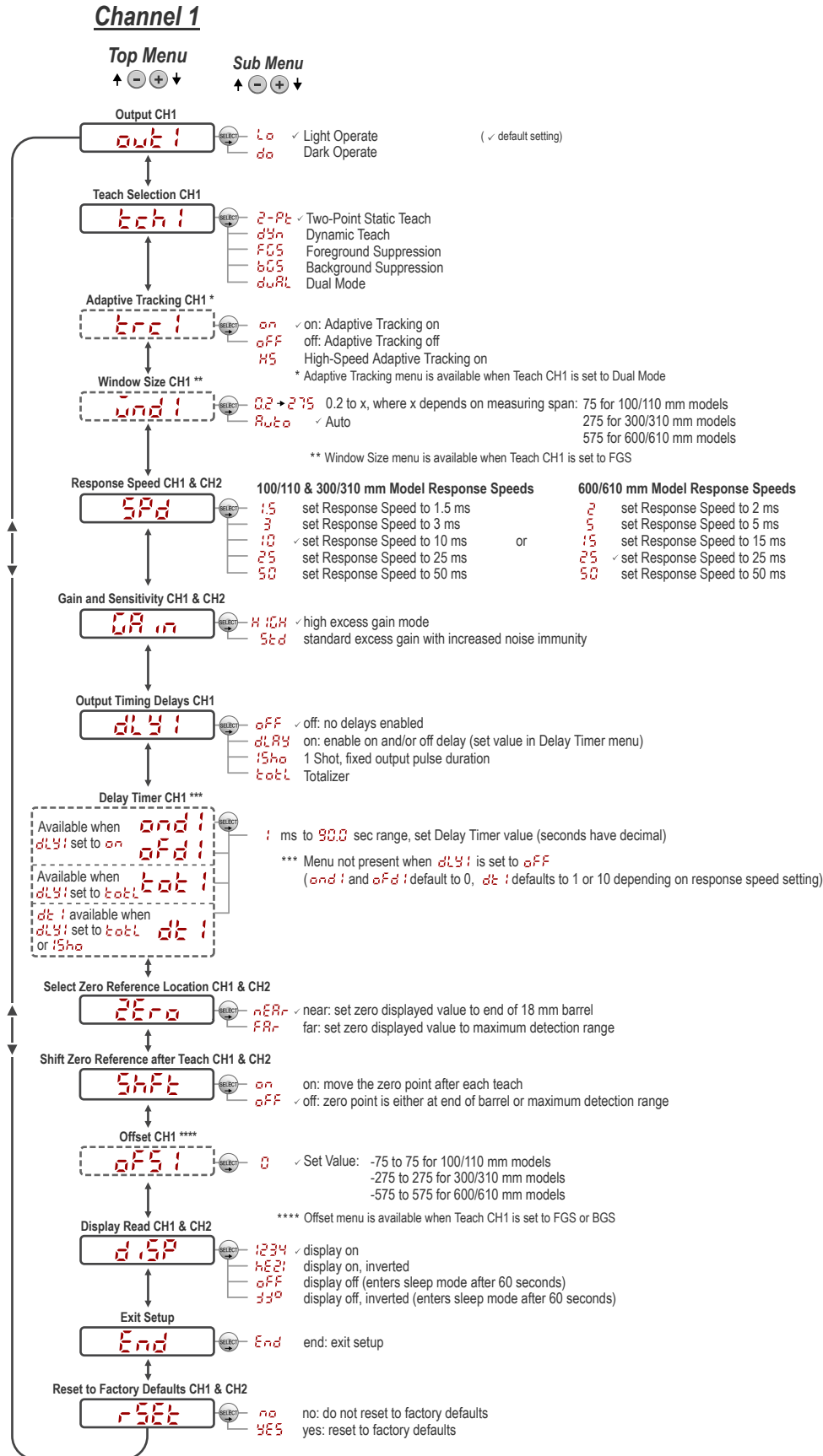
Figure 13. Sensor Menu Map—Channel 1
