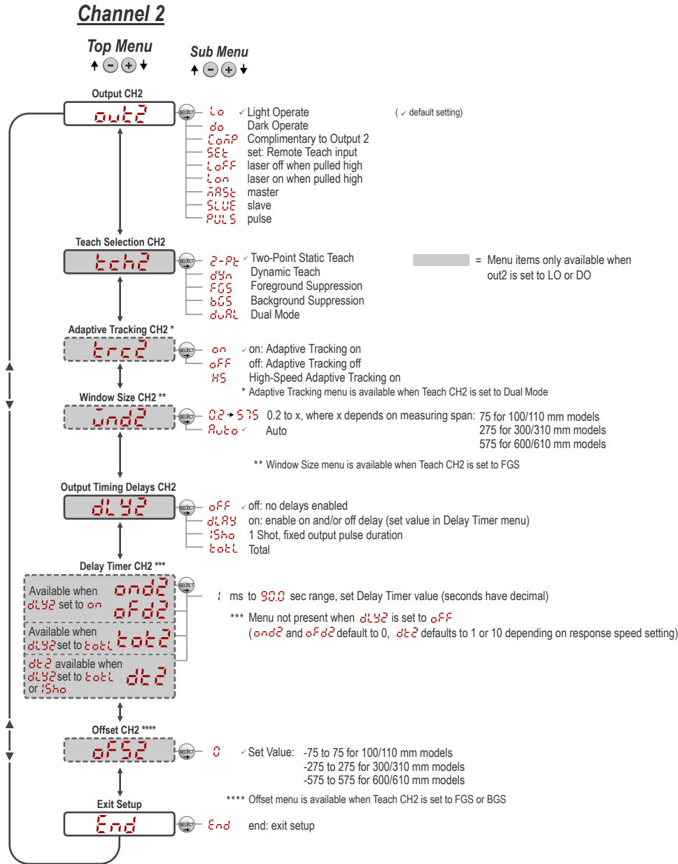
Figure 14. Sensor Menu Map—Channel 2
