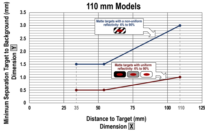
Figure 16. Minimum Object Separation Distance (90% to 6% reflectance)
