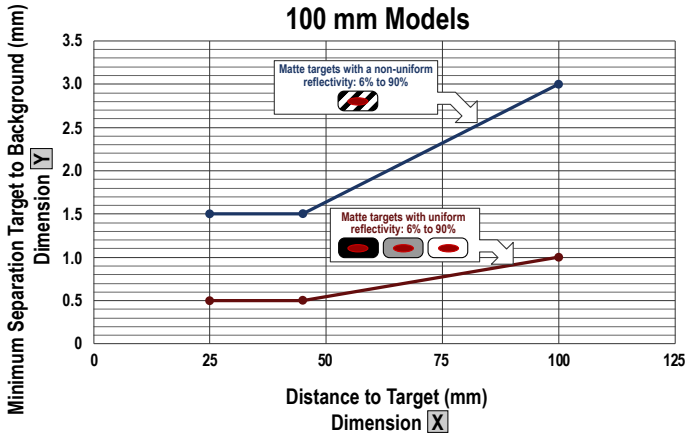
Figure 15. Minimum Object Separation Distance (90% to 6% reflectance)
